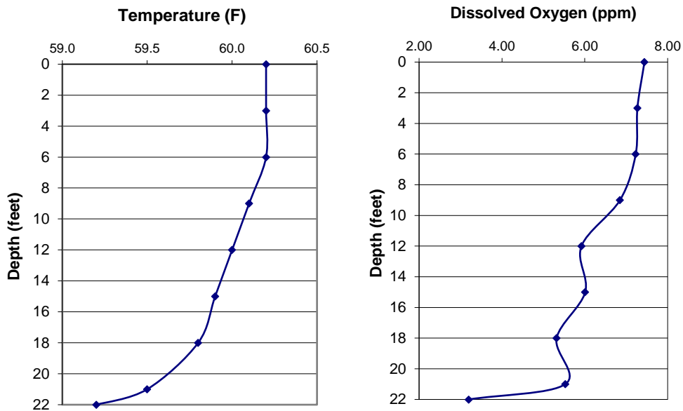
Figure 1: Temperature and oxygen profiles for Aquatic Control Pond, October 1, 2017.
